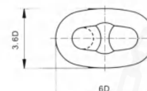
COMMON LINK=C (普通链环)
