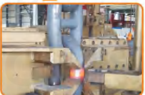
↑ 去刺 Trimming
