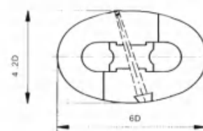
KENTER SHACKLE=KS (肯特卸扣)
