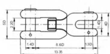
ANCHOR SWIVEL SHACKLE (b)=A.S.W.S (b) (B型转环卸扣)
