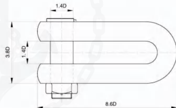
LTM END JOINING SHACKLE = LTM EJS (LTM 末端连接卸扣)
