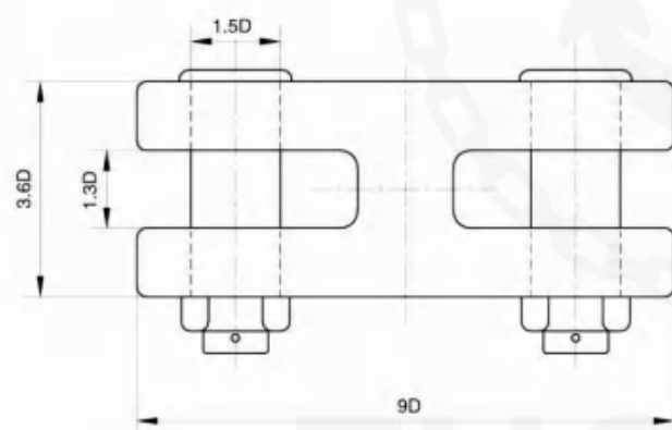
LTM H-TYPE JOINING SHACKLE = LTM HJS (LTM H型连接卸扣)
