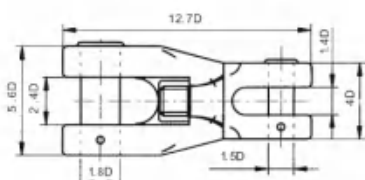
ANCHOR SWIVEL SHACKLE (a)=A.S.W.S (a) (A型转环卸扣)
